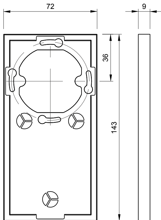
drawing the mounting plate
